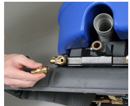
Quick change nozzle provides easy clean up and maintenance. The large opening dramatically reduces the potential for clogging.
